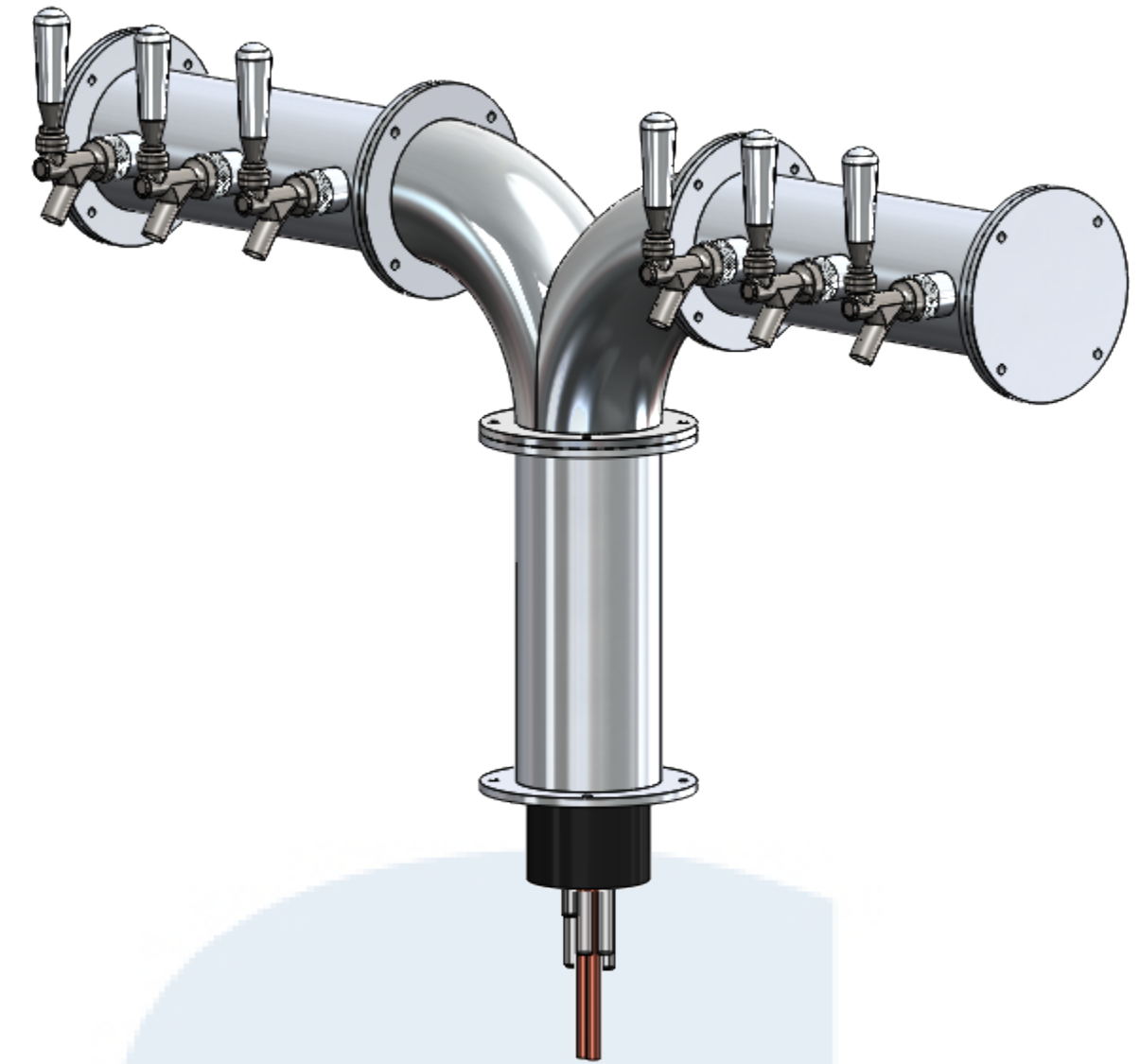
Isometric View (For reference purpose only)
